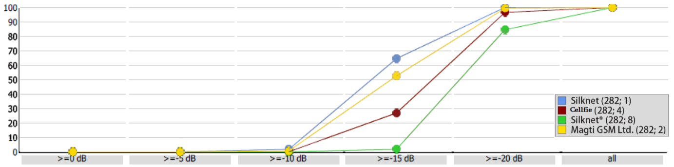
The chart below shows the cumulative distribution of the Top1 Interference samples (RSRQ) of different operators based on narrowband values
