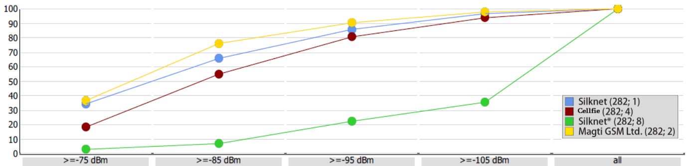
The chart below shows the cumulative distribution of the Top1 Coverage samples (RSRP) of different operators based on narrowband values
